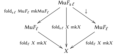
Figure 9. Proof of Lemma C.4
